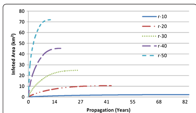
Figure 10 Spread of infected area due to AP radius (London).
