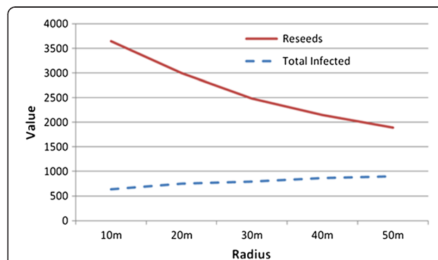
Figure 1 WiFi virus reseeding value versus total infected nodes for all radii (Belfast).
