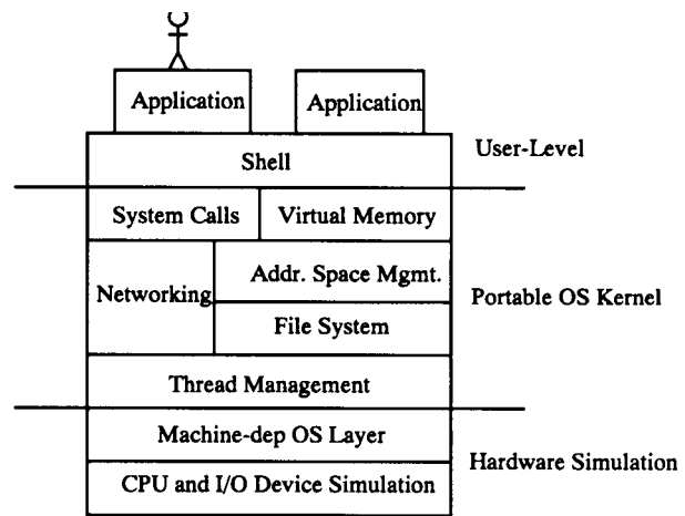
Figure 1: Nachos Software Structure
