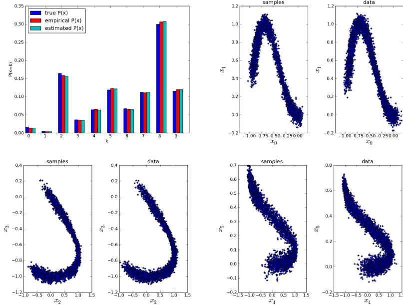
Figure 3: Top left: histogram of a data-generating distribution (true, blue), the empirical distribution (red), and the estimated distribution using a denoising maximum likelihood estimator. Other figures: pairs of variables (out of 10) showing the training samples and the model-generated samples.
