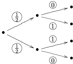
Figure 4.4: pasted probability
