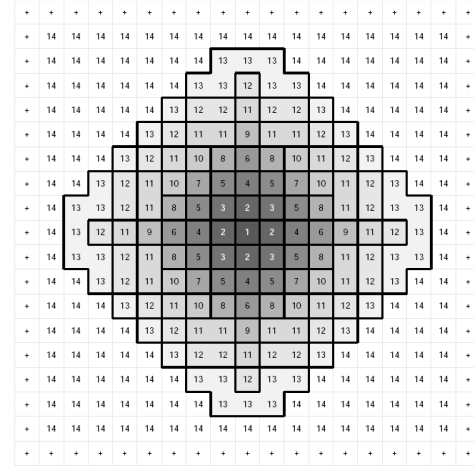
Fig. 1: Shape-Pattern templates of sizes 1 to 14 (Source: [9])
