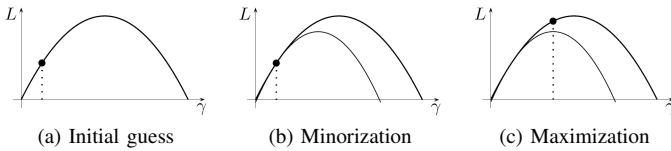
Fig. 2: Minorization-Maximization (Source: [5])
