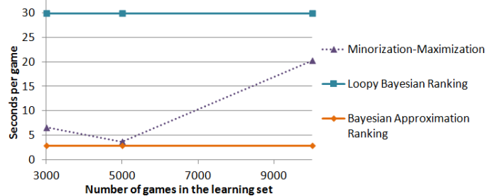
Fig. 10: Time needed per game on different training set sizes
