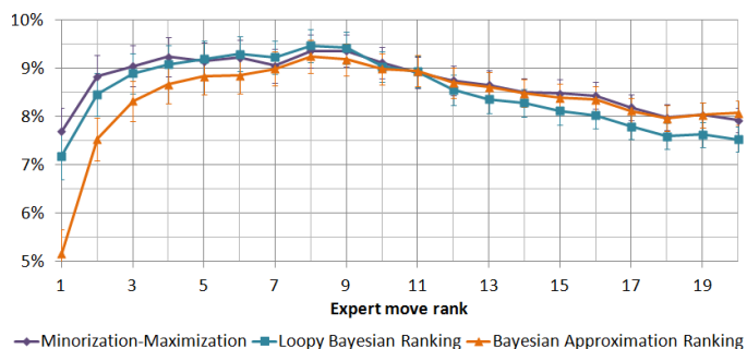
Fig. 6: Difference of cumulative prediction rank distribution to probabilistic ranking distribution. (95% conf. intervals)
