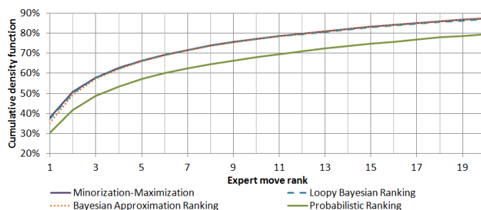
Fig. 5: Cumulative distribution of finding the expert move within the first n ranked moves.
