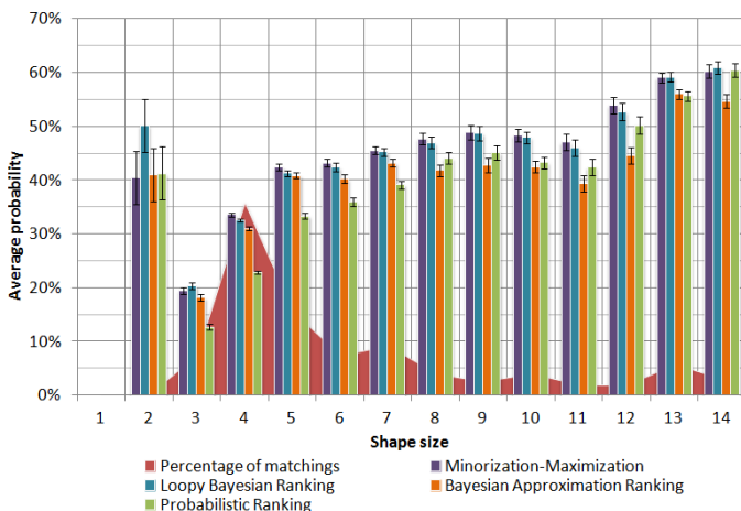
Fig. 8: Average prediction rates in relation to the size of the pattern that was matched at the expert move.
