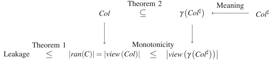
Figure 2: Relationship of collecting semantics Col , abstract fixpoint Col^\sharp , side channels C , and leakage bounds.
