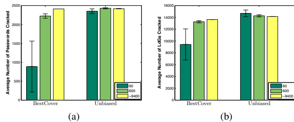
Figure 9: (a) Average number of passwords cracked vs. different training data sizes. (b) Average number of LdGs cracked vs. different training data sizes. P^2_{A-40} is used for this analysis. Average over 3 analyses, with one standard deviation shown.
