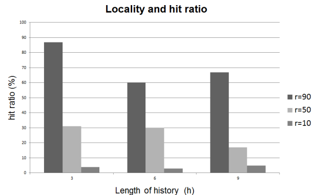
Figure 10: Whitelist LRU test results: X-axis of graph indicates parameter h , length of history locality, and the legend indicates the parameter r , the rate of locality. Y-axis of the graph shows the hit ratio.
