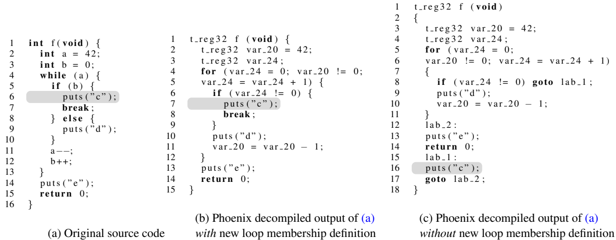
Figure 5: Loop refinement with and without new loop membership definition.
